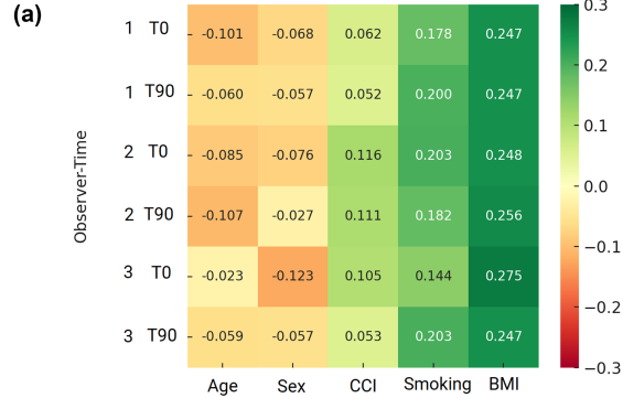
Correlation of TNM classification with Age, Sex, CCI, Smoking and BMI
