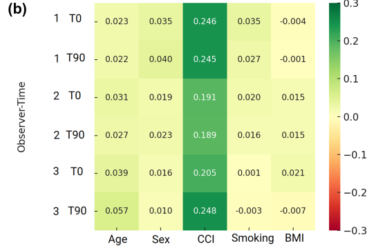
Figure 2. (a) Correlation of TNM classification with age, sex, CCI, smoking, and BMI in acute PJIs. (b) Correlation of TNM classification with age, sex, and Charlson comorbidity index in chronic PJIs.
