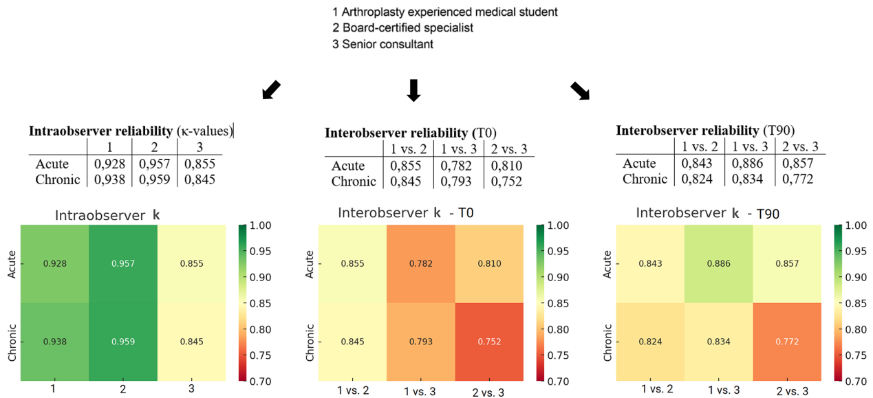
Figure 1. Intra-observer and inter-observer reliability (κ values) at time point 0 (T0) and after 90 d (T90).
