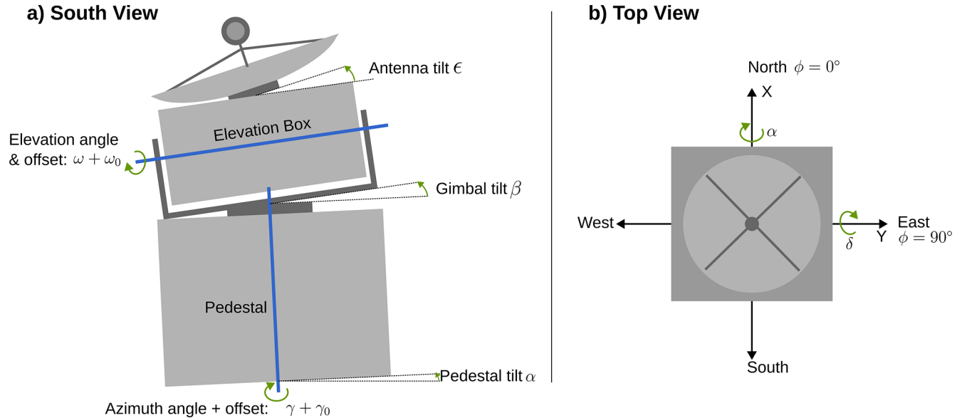
Figure 2. Inaccuracies of the scanner leading to beam pointing offsets, with the axes positioned at \gamma = 0^\circ and \omega = 90^\circ . (a) View from the South. (b) View from the top. The sign convention of each parameter is indicated by green arrows, which point into the positive direction of movement. Positive \alpha tilts the radar West, positive \delta tilts the radar North. Positive \gamma tilts the dish clockwise, if viewed from the top. For \gamma = 0^\circ and \omega = 0^\circ , the dish points to the North. For \gamma = 0^\circ , positive \omega tilts the elevation box clockwise, if viewed from the West.
