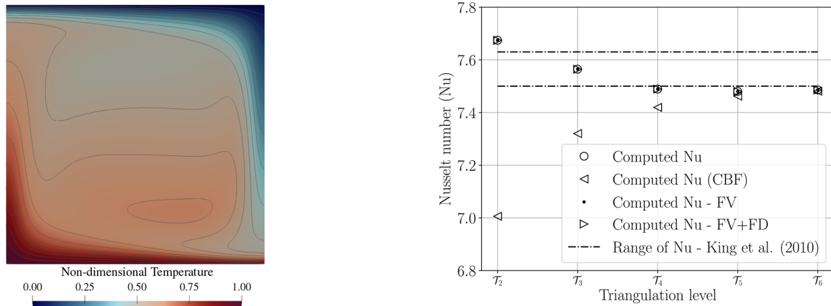
Figure 3. Left panel: final temperature contours of the compressible benchmark on an unit square of the TALA case from King et al. (2010) presented in Sect. 4.2.1 with Ra = 10^5 and Di = 0.5 ; right panel: comparison of Nusselt number values between the Frozen velocity approach (FV, see Sect. 2.3.1) and including Frozen divergence approach (FD, see Sect. 2.3.2) under the setup from Sect. 4.2.1 identical to the TALA case from King et al. (2010) at Ra = 10^5 and Di = 0.5 .
