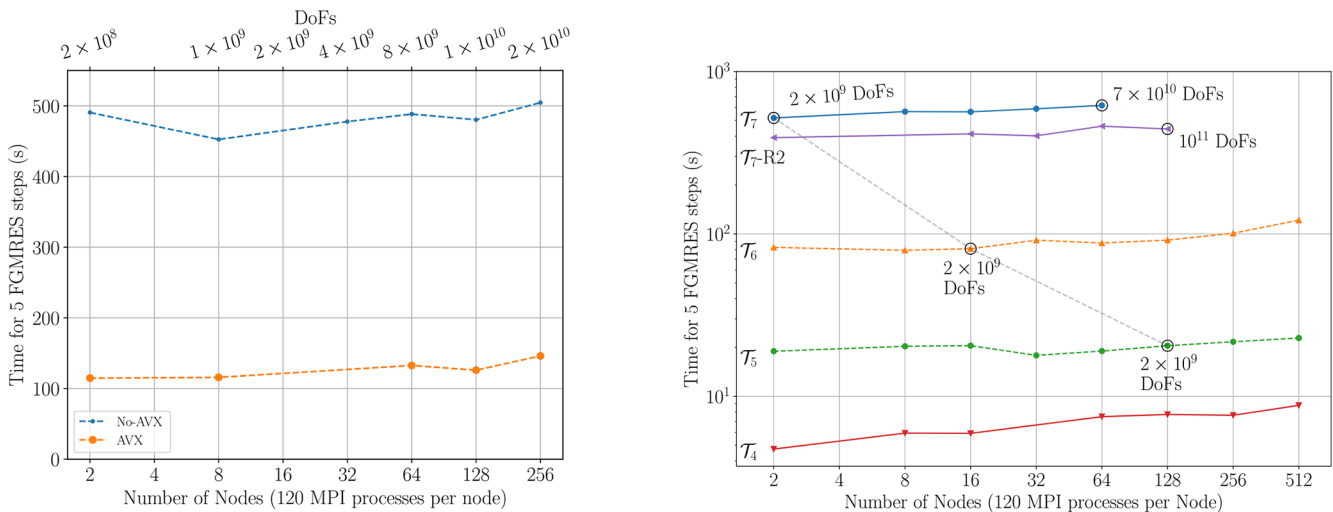
Figure 9. Left panel: weak scaling at T_6 for an identical setup with and without vectorization using the code generated from the HOG generator, right panel: weak scaling behaviour on the Hawk supercomputer at HLRS (66th on Top500 as of November 2024) up to 512 nodes; T_4 , T_5 , T_6 or T_7 gives the highest refinement level when simulating the variable viscosity Stokes system; the postfix-R2 indicates a weak scaling test with peak number of unknowns being 10^{11} (but a restart of FGMRES after already two steps due to memory limitations).
