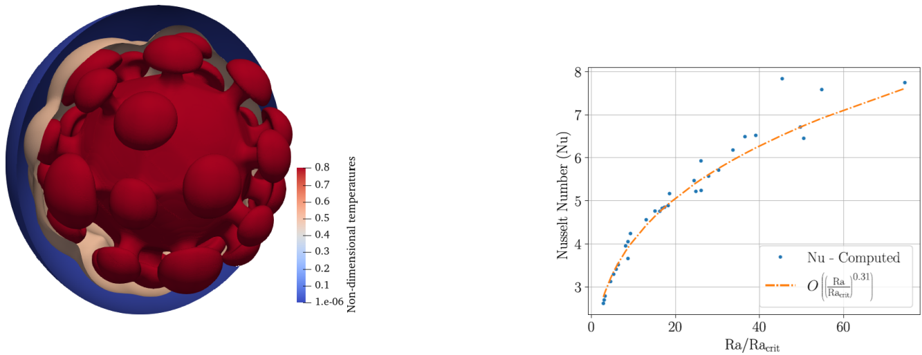
Figure 8. Left panel: temperature isosurfaces at T = 0.8 (red), T = 0.5 (light red) and T = 10^{-6} (blue) for the A7 case from Zhong et al. (2008); right panel: variation of Nu vs. (Ra/Ra_{crit}) for the cubic symmetry case; each data point denotes a simulation run where Ra_{crit} is computed depending on the r_\mu value for a given spherical harmonic perturbation, with the best fit exponent plotted side by side (Ra/Ra_{crit})^{0.31} .
