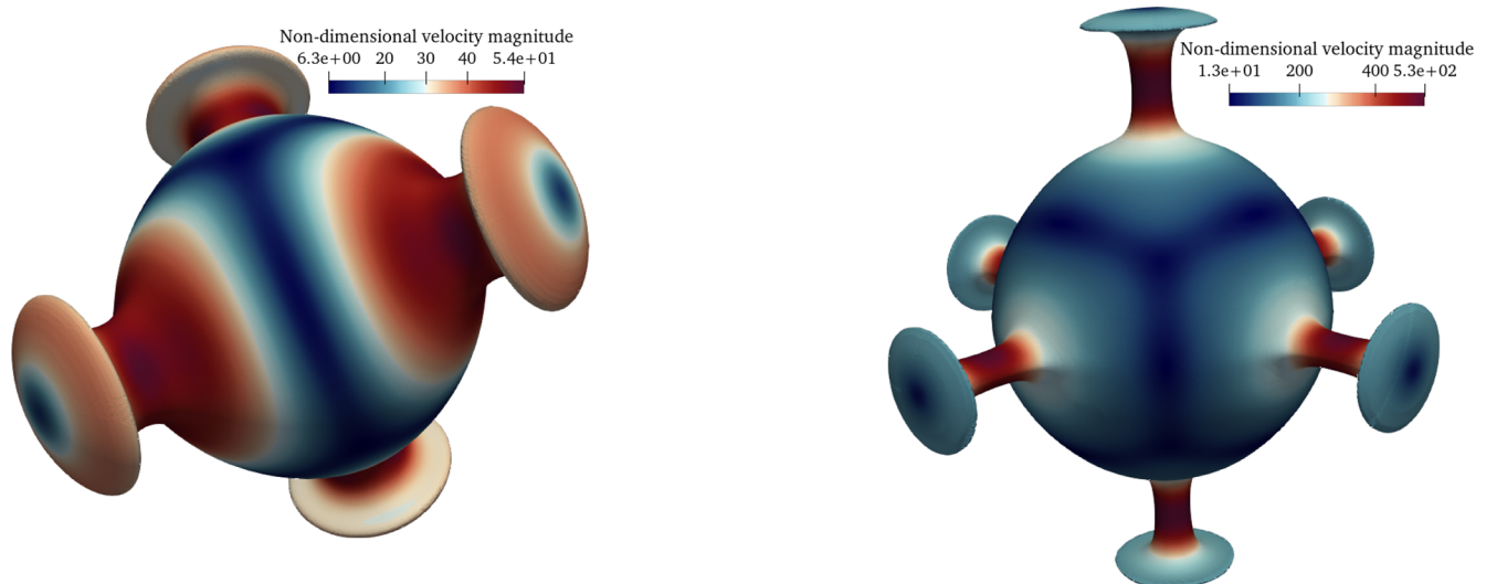
Figure 5. Left panel: temperature isosurfaces at T = 0.5 for the A3 case coloured with non-dimensional velocity magnitudes; right panel: temperature isosurfaces at T = 0.5 for the C3 case coloured with non-dimensional velocity magnitudes.
