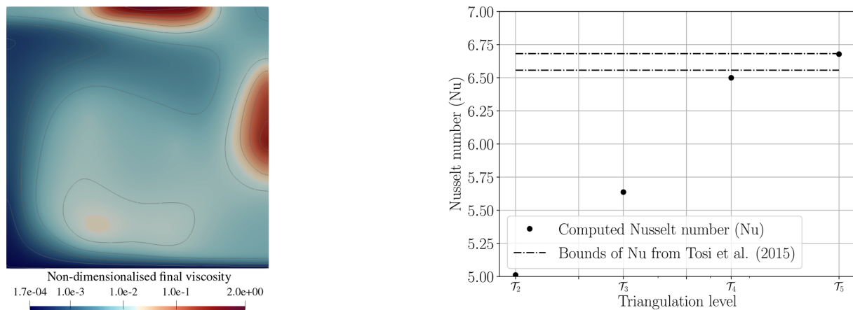
Figure 4. Results for the setup described in Sect. 4.2.2 after reaching steady state: left panel: final viscosity contours showing formed weak zones; right panel: convergence of the Nusselt numbers computed on the top boundary with mesh refinement.
