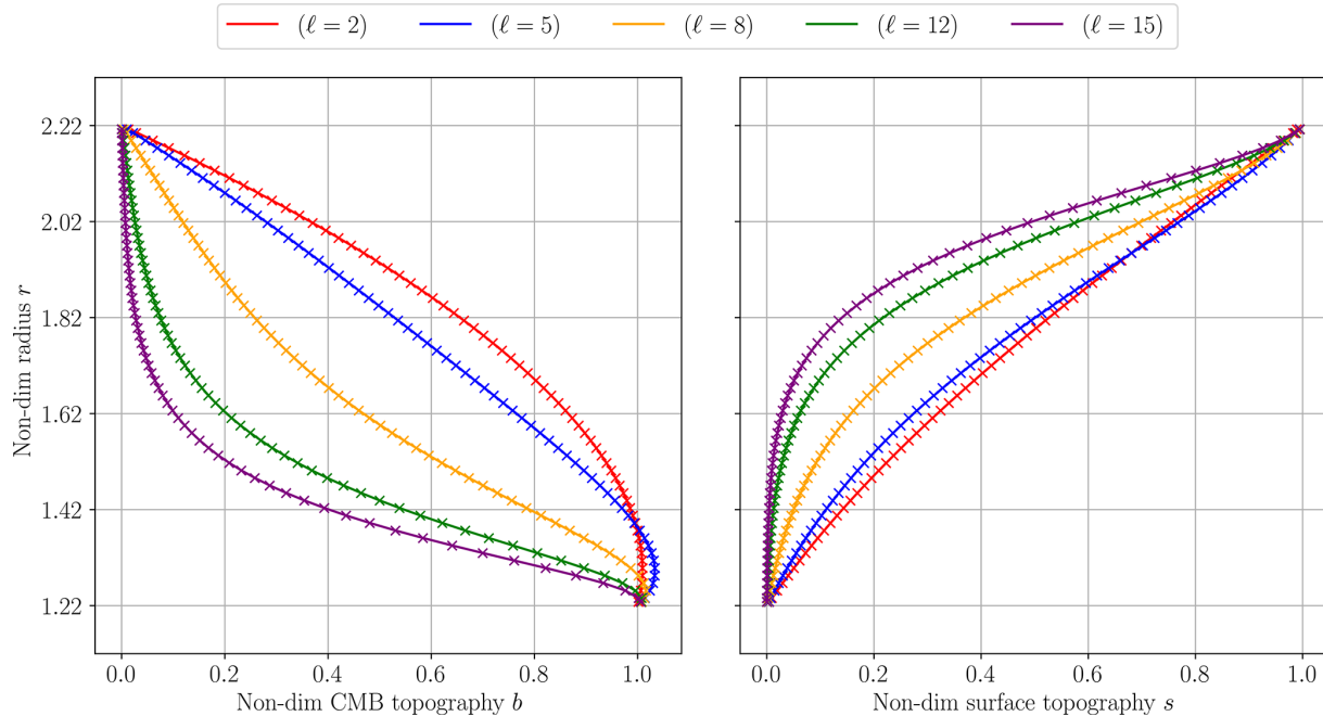
Figure 2. Kernels for the response of the surface and CMB topography to a \delta -function forcing of the specified spherical harmonic degree ( \ell ) placed at various depths in the mantle; solid lines denote the analytical solution and the cross marks (x) denote the FE computed solution.
