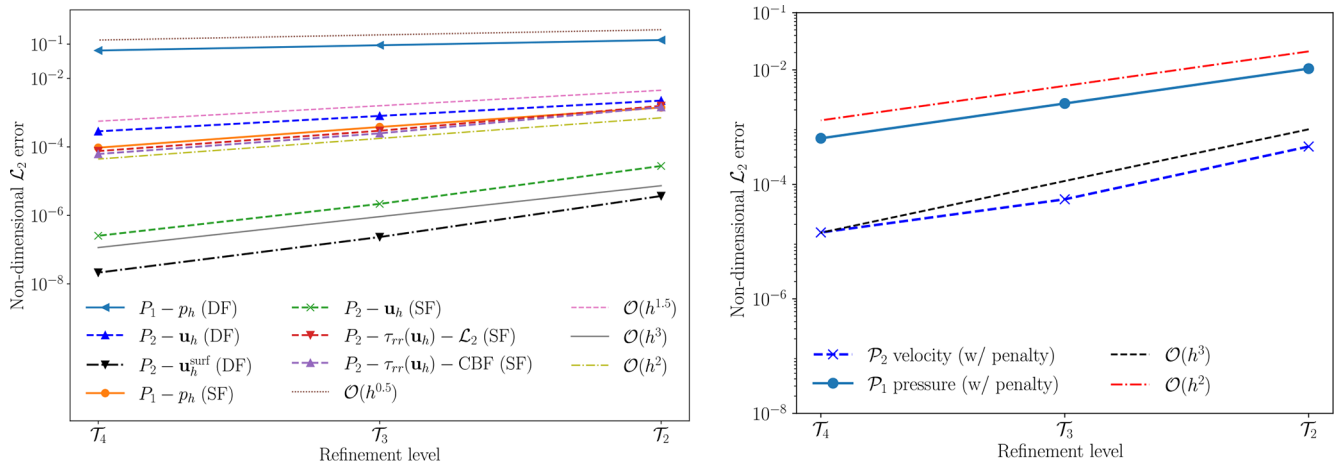
Figure 1. Left panel: order of convergence of the P_2 – P_1 FE solution to analytical solution on the Spherical Shell with noslip condition on outer and free-slip on the inner surface (mixed case) under the \delta -forcing (denoted by DF) function case and smooth-forcing (denoted by SF) function case for (\ell = 2, m = 2) , for SF case k = 2 ; right panel: order of convergence of the P_2 – P_1 FE solution to analytical solution on the Spherical Shell with free-slip imposed on both surfaces under the smooth forcing case and tuned rotational mode penalty for (\ell = 2, m = 2, k = 2) .
