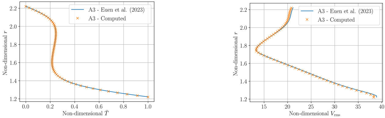
Figure 6. Radially averaged temperature values \bar{T} (left panel) and radially averaged velocity RMS values V_{\text{rms}} (right panel) for the A3 case from Zhong et al. (2008); we compare the results published in Euen et al. (2023) (solid line) with results computed in our setup.
