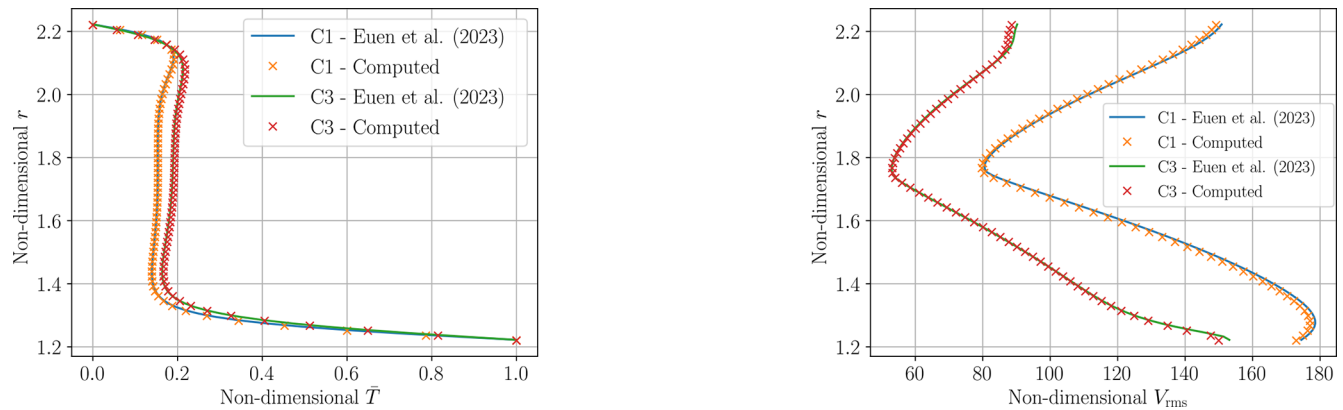
Figure 7. Radially averaged temperature values \bar{T} (left panel) and radially averaged velocity RMS values V_{\text{rms}} (right panel) for the C1 and C3 cases from Zhong et al. (2008); we compare the results published in Euen et al. (2023) (solid lines) with results computed in our setup.
