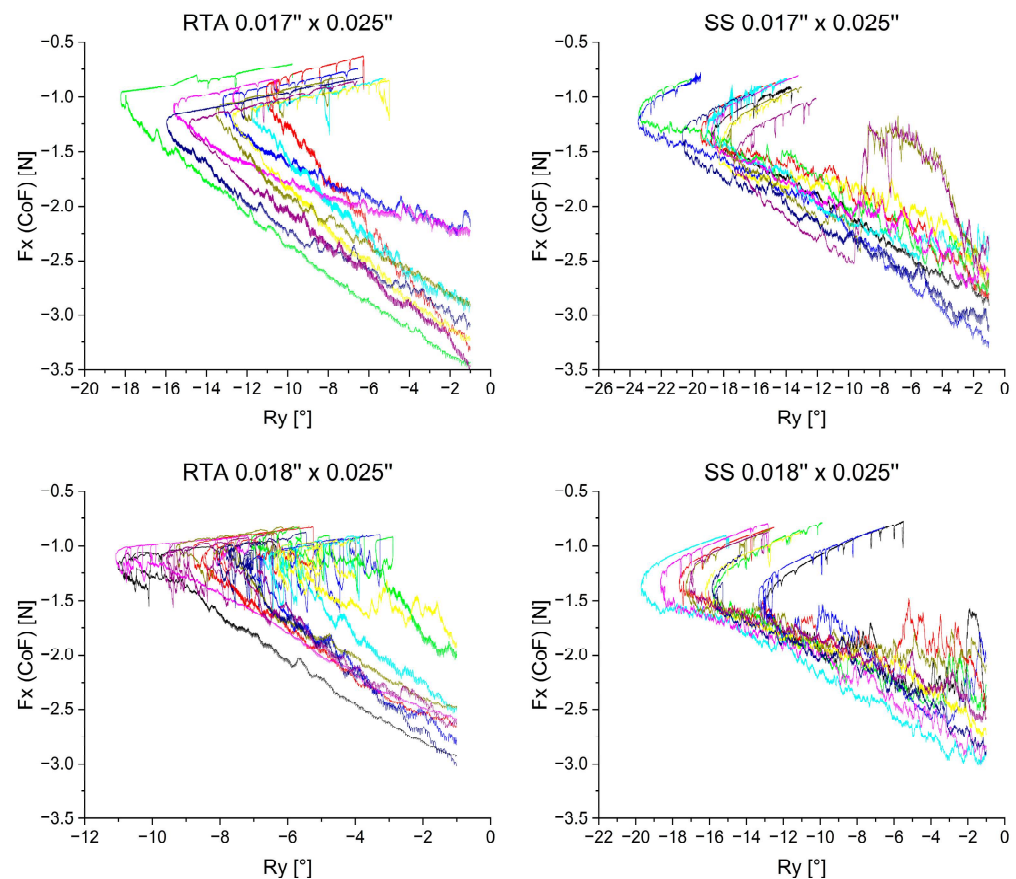
Figure 5. Retractive force F_x measured in the center of resistance plotted against the rotation angle of the anterior segment. The different colors represent different archwires. To account for initial irregularities, initial force values are depicted after -1^\circ of rotation. While the ordinate is the same in all graphs, the abscissa, with the rotational angle R_y has a variable resolution.
