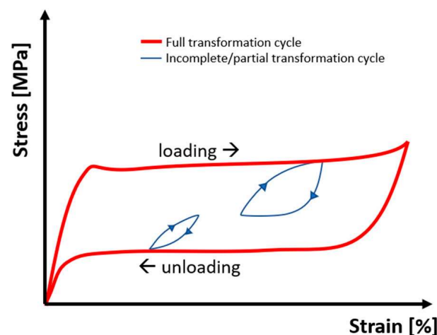
Figure 9. Schematic depiction of the stress-strain behavior of superelastic NiTi alloys in case of interrupted loading or unloading cycles [35].
