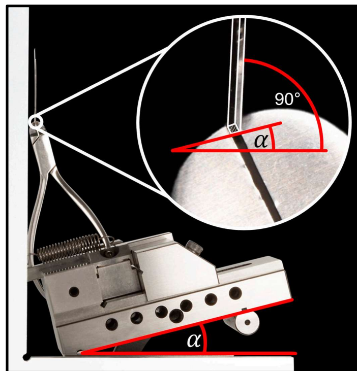
Figure 2. Torque measurement device. A tweed forceps was mounted on an adjustable parallel vice. After aligning the table using the clamped archwire parallel to 90^\circ angle of the table plane, the anterior torque \alpha (°) can be measured using a digital angle meter.
