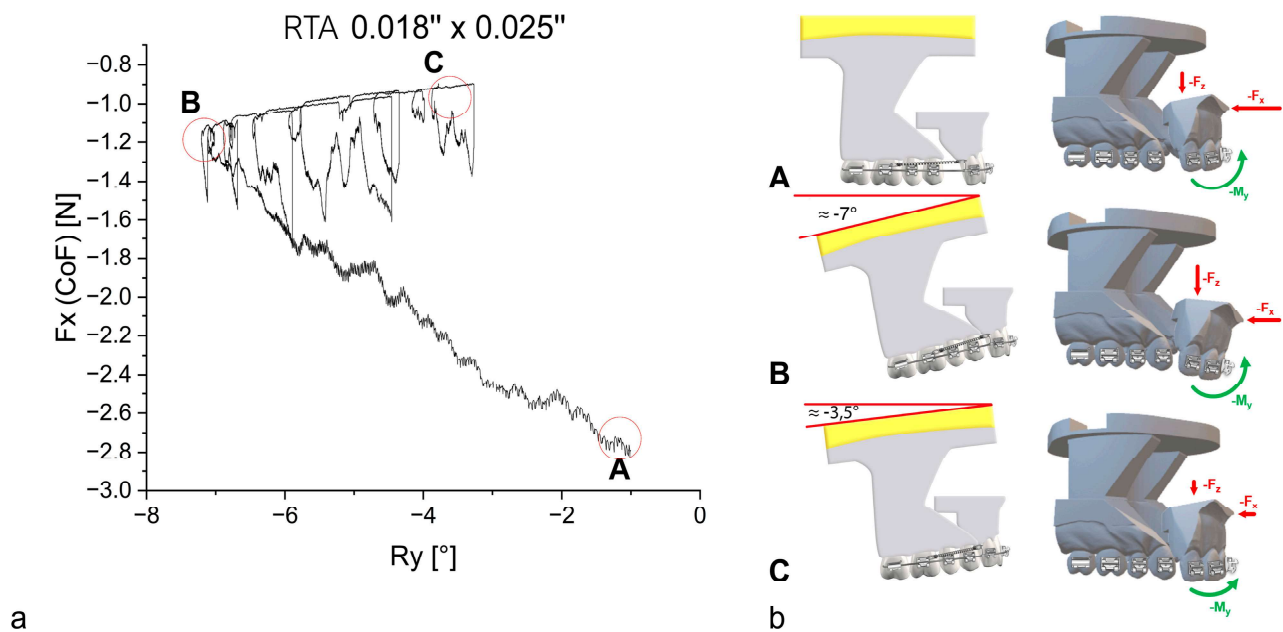
Figure 6. (a) The retractive force F_x is plotted against the rotation of the anterior segment of teeth for an 0.018'' \times 0.025'' RTA. In order to reduce preliminary irregularities, initial force values are depicted after -1^\circ of rotation. (b) Correlating graphics of the experimental model segments at the different time points (A, B, C) of en-bloc retraction. The rotating posterior segment is being moved by the hexapod device, while the anterior segment is statically fixed to the force-torque sensor, which represents an inversion of the in vivo process, showing force and moment vectors ( F_x , F_z and M_y ) on the anterior tooth segment. The lengths of the vectors represent the force and torque values schematically.
