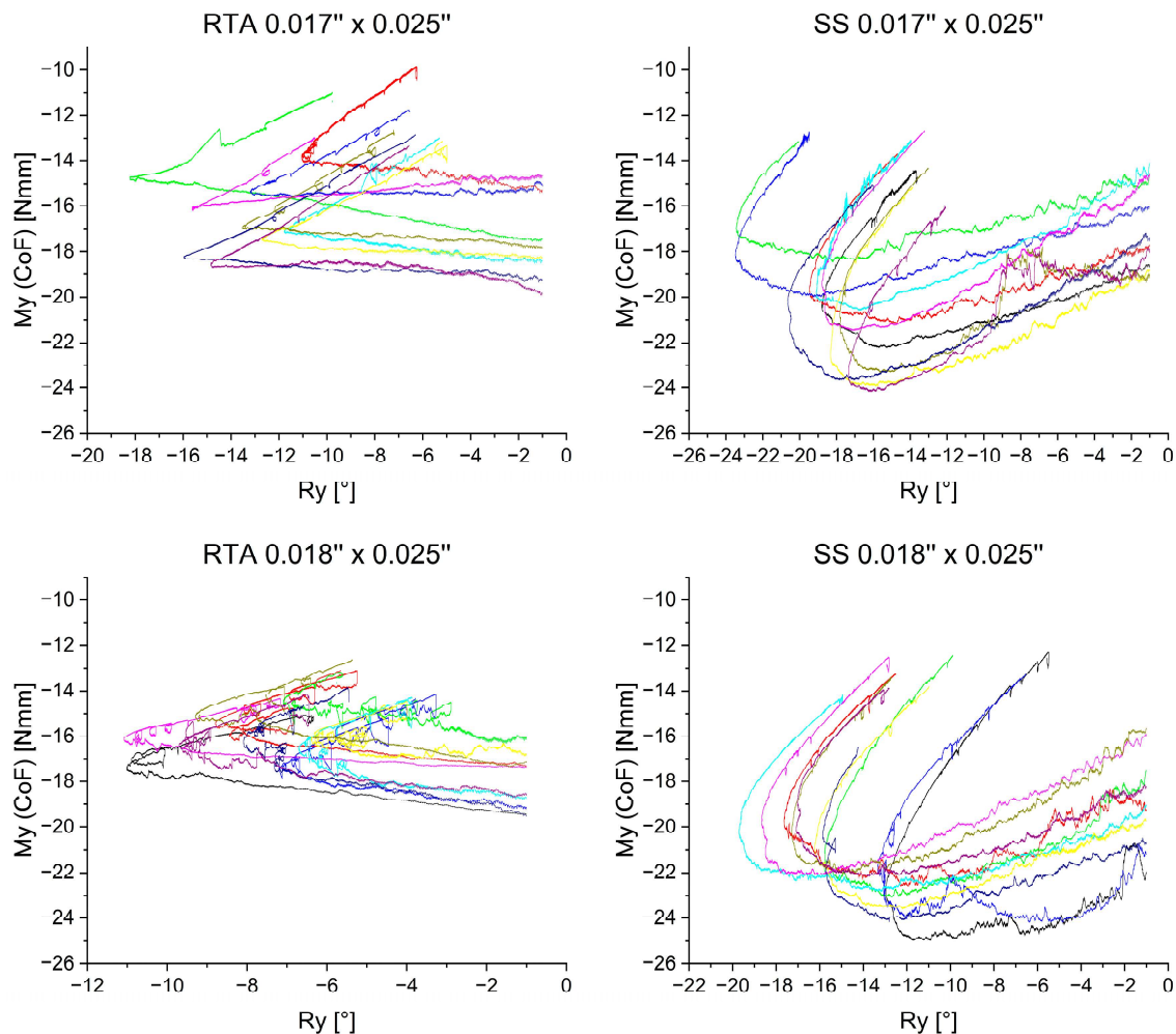
Figure 7. Rotational moment M_y measured in the center of resistance plotted against the rotation of the anterior segment. The different colors represent different archwires. To reduce preliminary irregularities, initial rotational moment values are depicted after -1^\circ of rotation. While the ordinate is the same in all graphs, the abscissa with the rotational angle R_y has a variable resolution.
