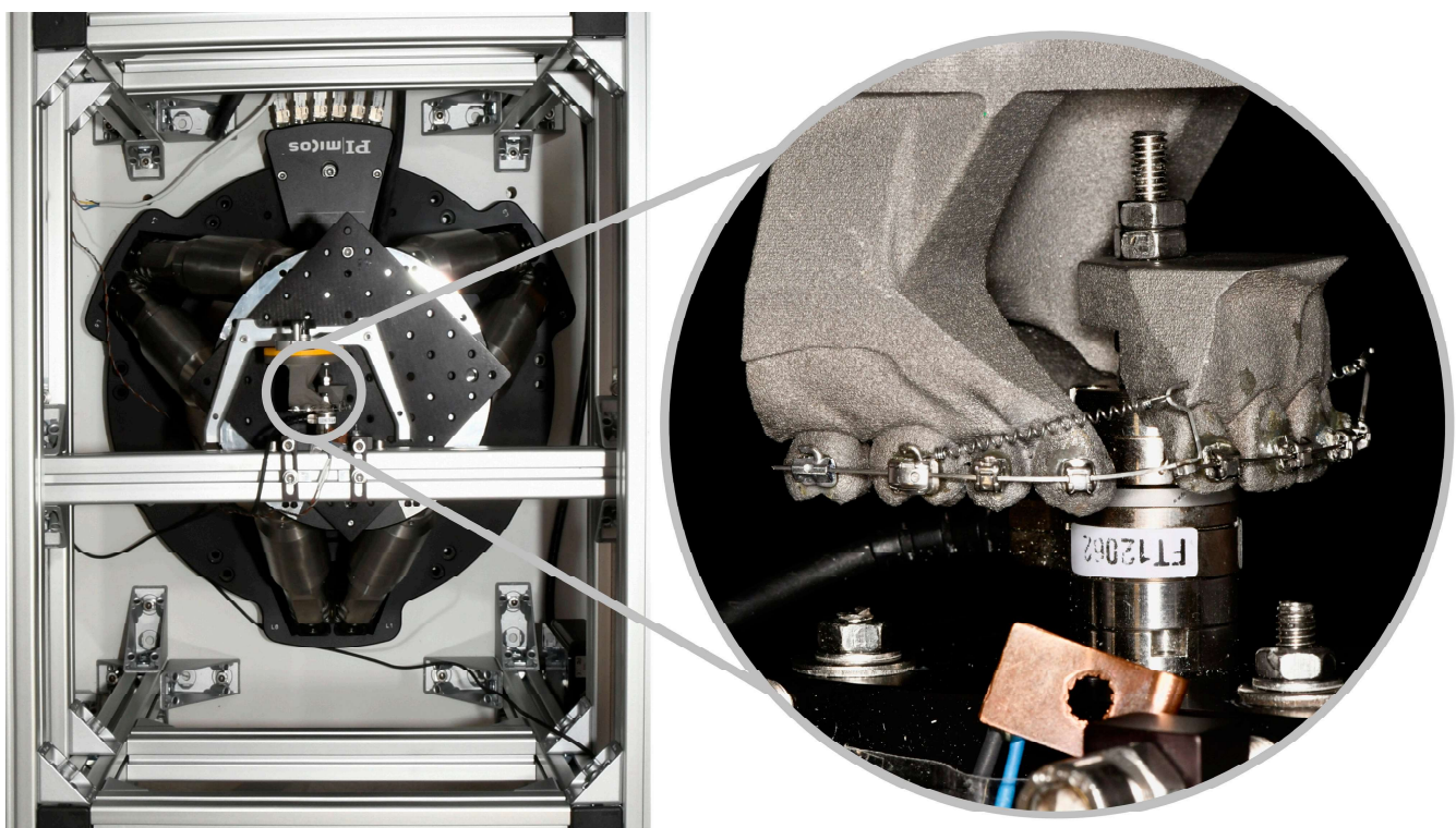
Figure 3. HOSEA's temperature-controlled experimental chamber. Six hydraulic legs of the hexapod move the connected Stewart platform and the posterior part of the experimental model. The close-up depicts both model parts mounted within the experimental set-up. The anterior part is rigidly attached to a cross strut and force-torque sensor.
