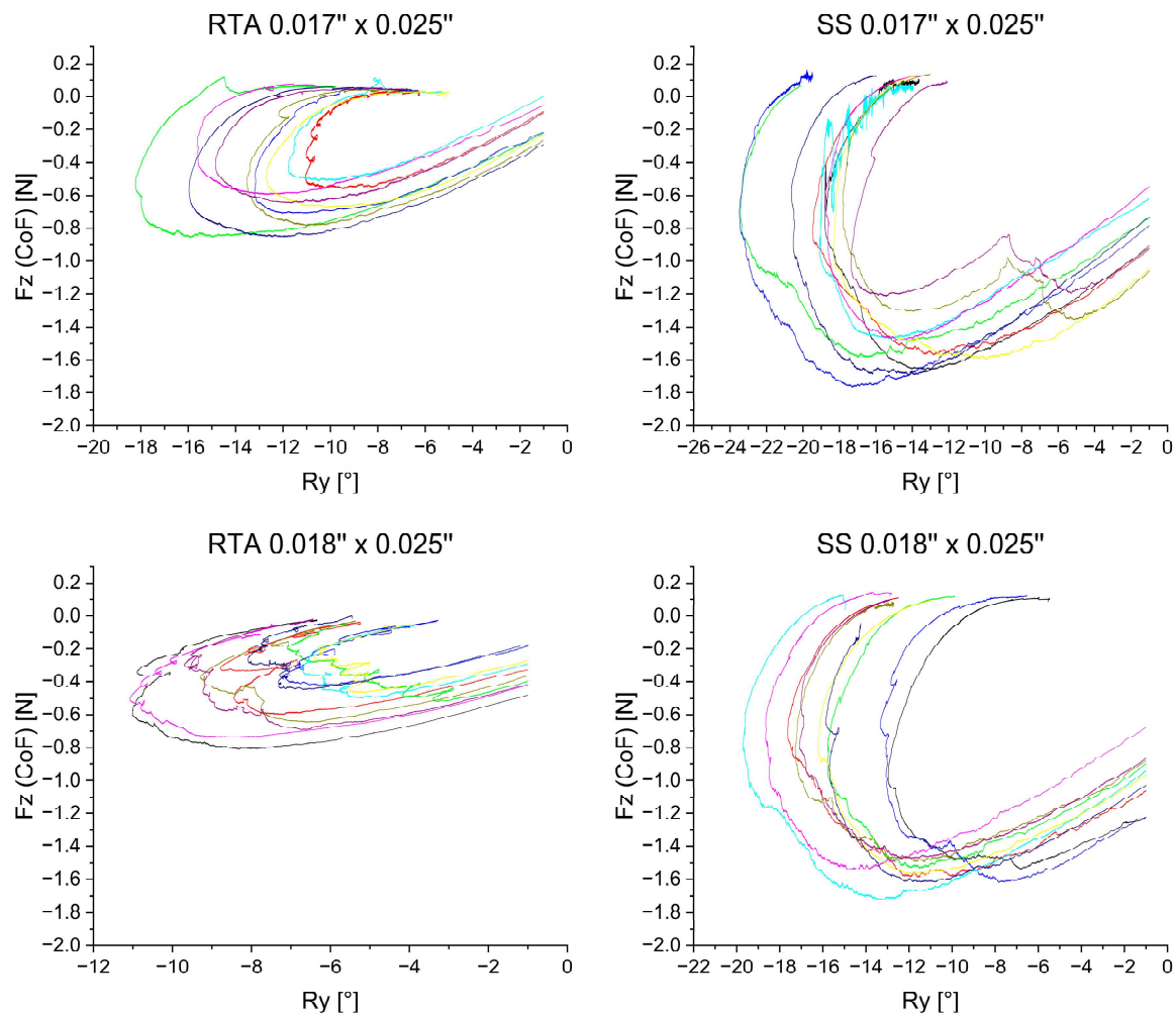
Figure 8. Extrusive force F_z measured in the center of resistance plotted against the rotation of the anterior segment. The different colors represent different archwires. To reduce preliminary irregularities, initial force values are depicted after -1^\circ of rotation. While the ordinate is the same within the material groups (RTA and SS), the abscissa with the rotational angle R_y has a variable resolution.
