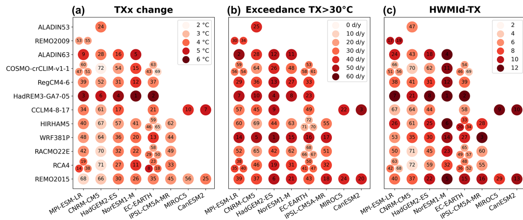
Figure 8. GCM–RCM matrix of EURO-CORDEX models for (a) the change in yearly maximum near-surface air temperature (TXx) between 1981–2010 and 3 °C European warming, (b) TX exceedances above 30 °C at 3 °C European warming, and (c) Heat Wave Magnitude Index daily based on TX (HWMid-TX) at 3 °C European warming. Each circle indicates the average value across all investigated cities for each individual EURO-CORDEX model. Numbers in the circle indicate the ranking of models from 1 (highest ambient heat) to 72 (lowest ambient heat). Multiple ensemble members for a GCM–RCM combination are indicated as smaller circles.
