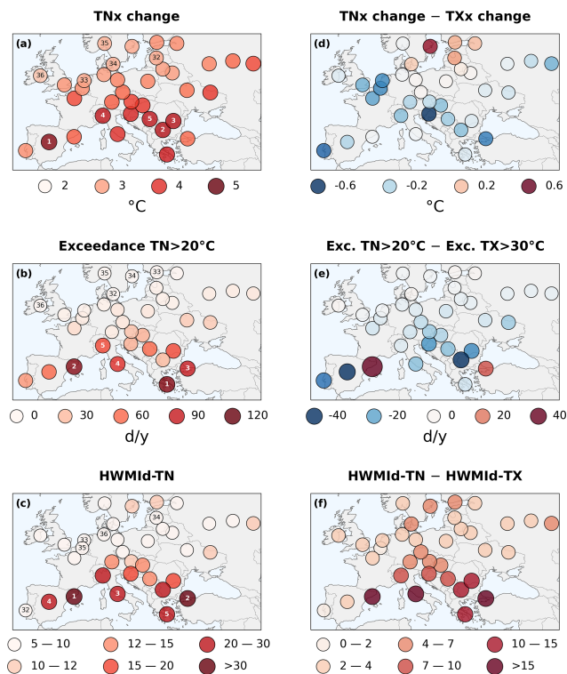
Figure 6. As in Fig. 4 but for daily minimum near-surface air temperature (TN) in panels (a)–(c). Panels (d)–(f) show the difference between ambient heat estimates based on TN and based on daily maximum near-surface air temperature (TX). Note that the scale for HWMid-TN differs from the HWMid-TX scale in Fig. 4.
