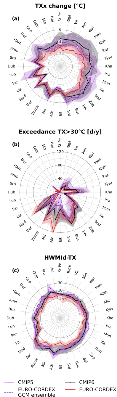
Figure 7. Projections of ambient heat in European cities for EURO-CORDEX, CMIP5, CMIP6, and the EURO-CORDEX GCM ensemble. Cities are arranged according to their geographical location, i.e. northern European cities at the top, eastern European cities on the right, southern European cities at the bottom, and western European cities on the left. (a) Change in yearly maximum near-surface air temperature (TXx) between 1981–2010 and 3 °C European warming, (b) TX exceedances above 30 °C at 3 °C European warming, and (c) Heat Wave Magnitude Index daily based on TX (HWMid-TX) at 3 °C European warming. Note the logarithmic axis for the HWMid-TX panel. Lines indicate the multi-model median and shading the interquartile range across models.
